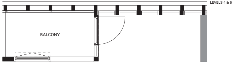
LEVELS 4 & 5
